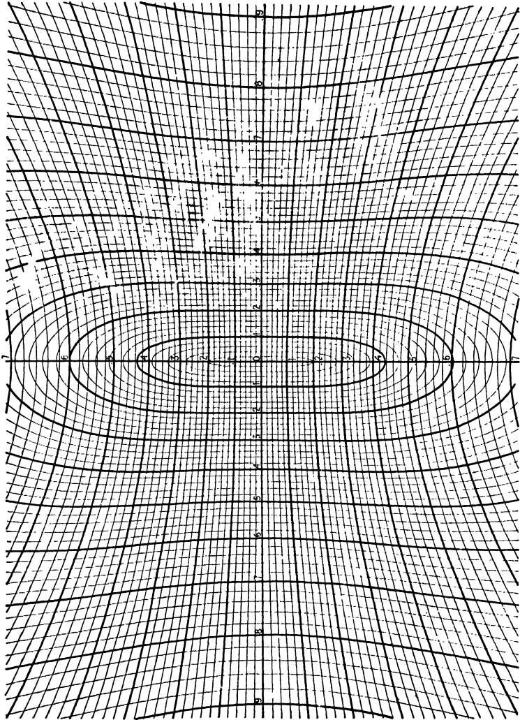
FIG. 20.—A chart for reading values of \xi and \zeta from a plane photographic plate. In the original chart the distance from crystal to plate is 10 cm. The length of the original chart is 11 in. (After Bernal.)
